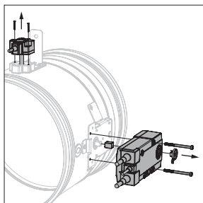
Type BFL(T) (-SR) on CR60/ CR120/CRS60/CU-LT(1s):
