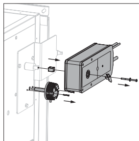
Type BLF(T) on CR2/CU2/CU4/CU2-15:
