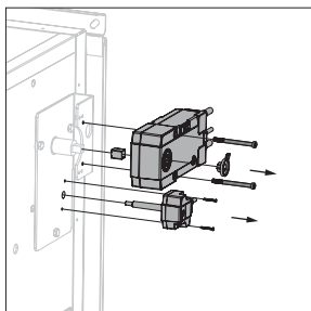
Type BFL(T) on CR2/CU2/ CU4/CU2-15:
