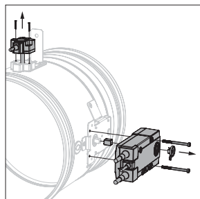
Type BFL(T) (-SR) op CR60/ CR120/CRS60/CU-LT(1s):
